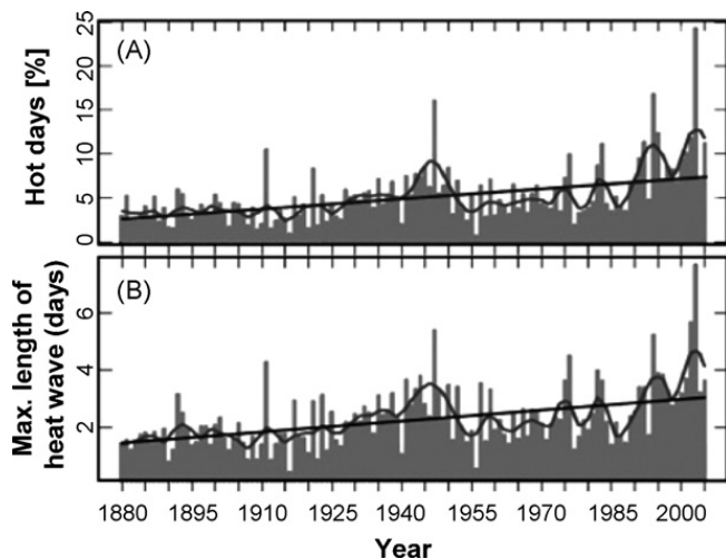
Fig. 2. Percentage of warm summer days (A) and the maximal length of heat waves (B) over the last 120 years. Data are based on sources from central European weather stations (modified from [12]).
