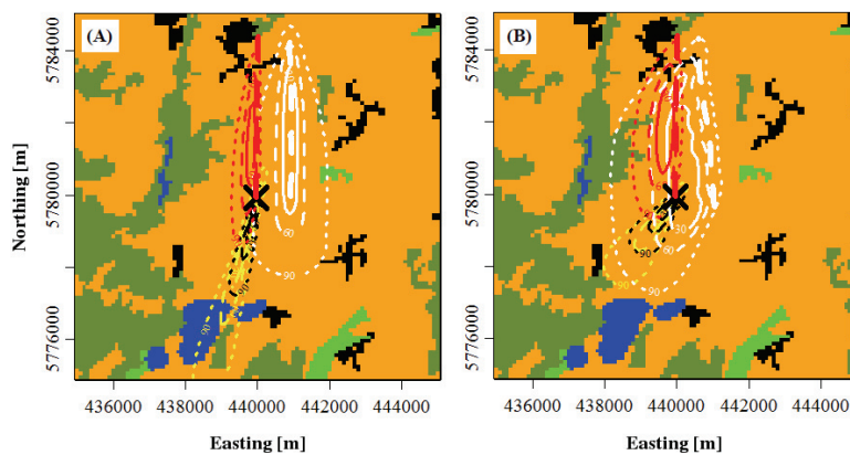
Fig. 9. Footprint effect levels of the measurements from Fig. 8 on 20 October 2008 (A) and 21 October 2008 (B) , presented similar to Fig. 7. In addition the weighted footprint along the LAS path is shown (red), and the footprint from the tower measurements at 50 m (black) and 90 m (yellow) are distinguished.
