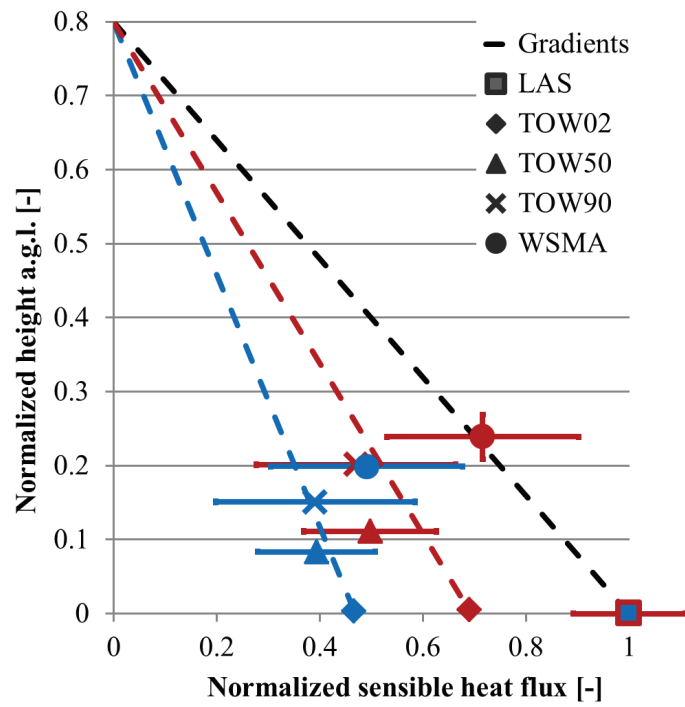
Fig. 8. Vertical profile of the sensible heat flux during two flights, 20 October 2008, 10:53–10:55 UTC (brown) and 21 October 2008, 09:56–09:59 UTC (blue). Heat fluxes are compared between large aperture scintillometer (LAS), tower eddy covariance at 2.4 m, 50 m and 90 m (TOW02, TOW50, TOW90) and the weight-shift microlight aircraft (WSMA). Where available, error bars show the random flux error and the altitude standard deviation. Additional information is given in the text.
