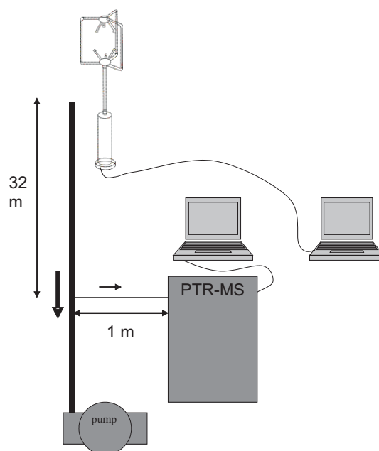
Fig. 1. Schematic of the measurement system. The black lines indicate Teflon tubing with flow direction indicated by arrows. The inner diameter of the long tubing was 8 mm and the flow in it 15 \text{ L min}^{-1} . The side flow of 0.1 \text{ L min}^{-1} was taken to the PTR-MS via tubing with 1.6 mm inner diameter.
