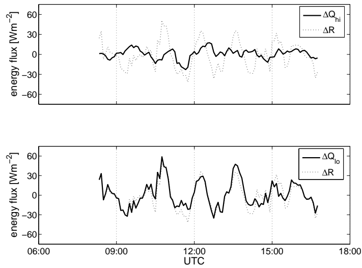
Fig. 1. Comparison of the change of the turbulent fluxes of sensible and latent heat in the high frequency range ( \Delta Q_{rghi} ) and the low frequency range ( \Delta Q_{lo} ) and the change of the residual of the energy balance closure ( \Delta R ) for 30 min averages determined for time steps of 5 min. A moving average (daily cycle) was subtracted (8 June 2003).
