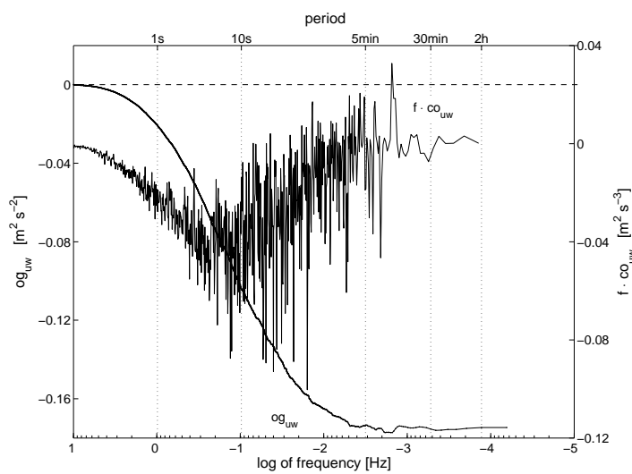
Fig. 2a. Ogiven (og) convergent within 30 min (Case 1) and co-spectrum (co), momentum flux on 9 June 2003 (12:30–16:30 UTC).
